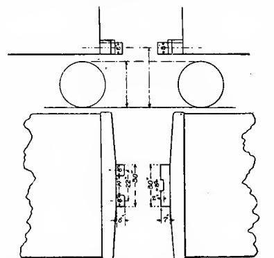
Fig. 5550-5551. THE LOCATION OF BUFFER BLOCKS AND BUFFER-BEAM.
